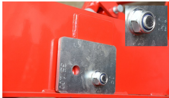
Ezi-Set height system with 6 etched height settings
