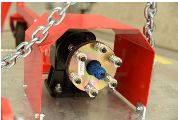
Clutch mounted to gearbox Heavy duty PTO guard
